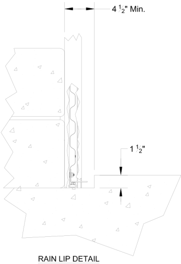
RAIN LIP DETAIL
