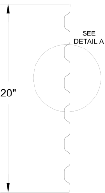
26 GA CURTAIN PANEL DETAIL
