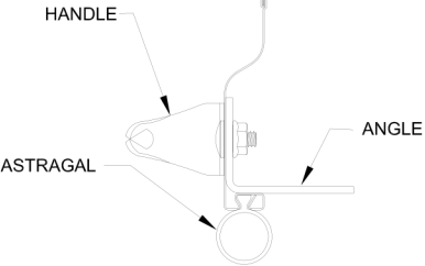
BOTTOM BAR ASSEMBLY
