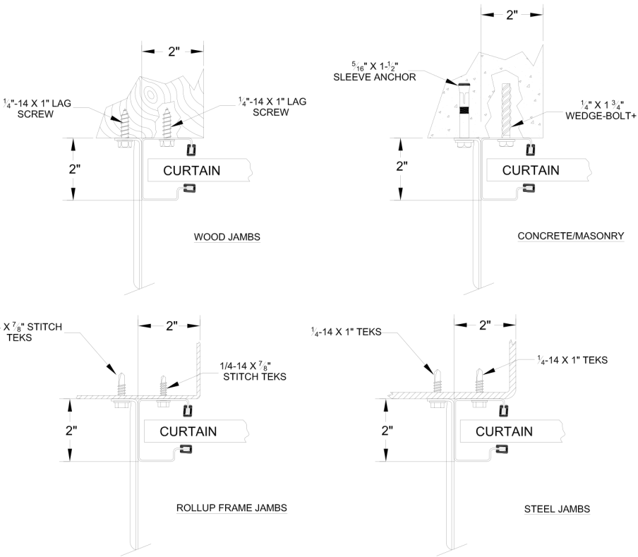
18 GA GUIDE & BRACKET MOUNTING DETAIL
